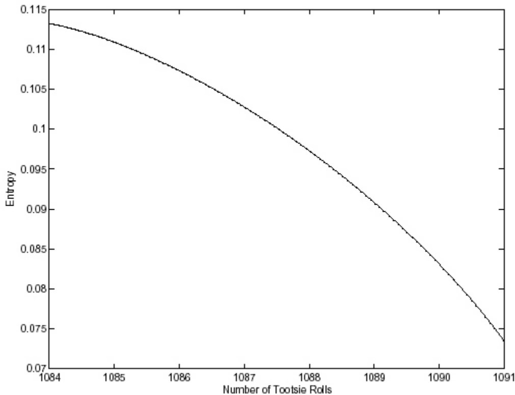
Figure 7-2: Entropy of the candy probability distribution
