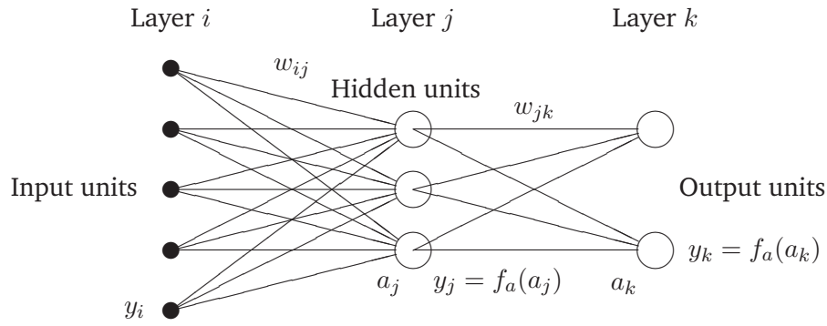
Figure 10: Schematic of a 5-3-2 multi-layer perceptron. Bias units and their weights are omitted for clarity.
