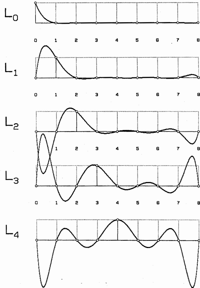
9-point closed NEWTON-COTES
