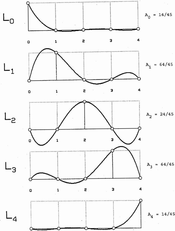
5-point closed NEWTON-COTES
