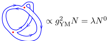
Figure 3: Non-planer graph that contributes to the vacuum \rightarrow vacuum amplitude.
