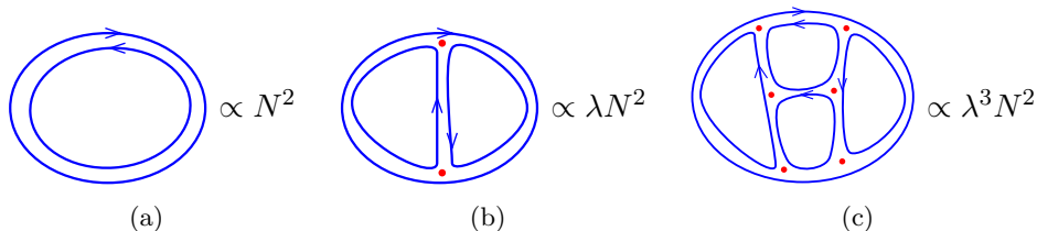
Figure 2: Planer graphs that contribute to the vacuum \rightarrow vacuum amplitude.
