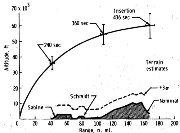
Figure 15. - Predicted Apollo 11 ascent dispersions.
