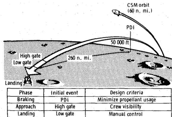
Figure 2. - Operational phases of powered descent.
