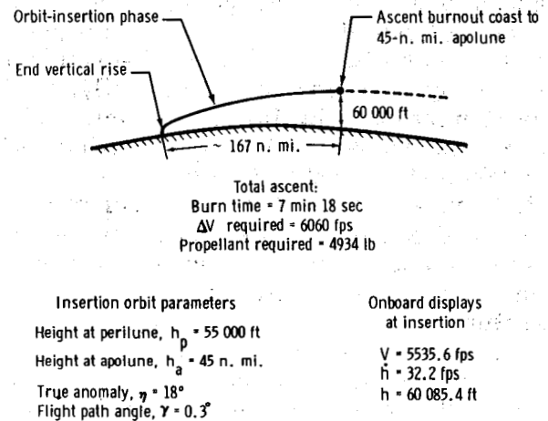
Figure 14. - Premission Apollo 11 orbit-insertion phase.
